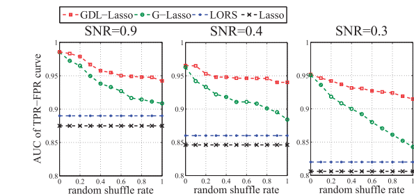
Fig. 5. The areas under the TPR-FPR curve (AUCs) of Lasso, LORS, G-Lasso and GDL. In each panel, we vary the percentage of noises in the prior networks S_0 and G_0
